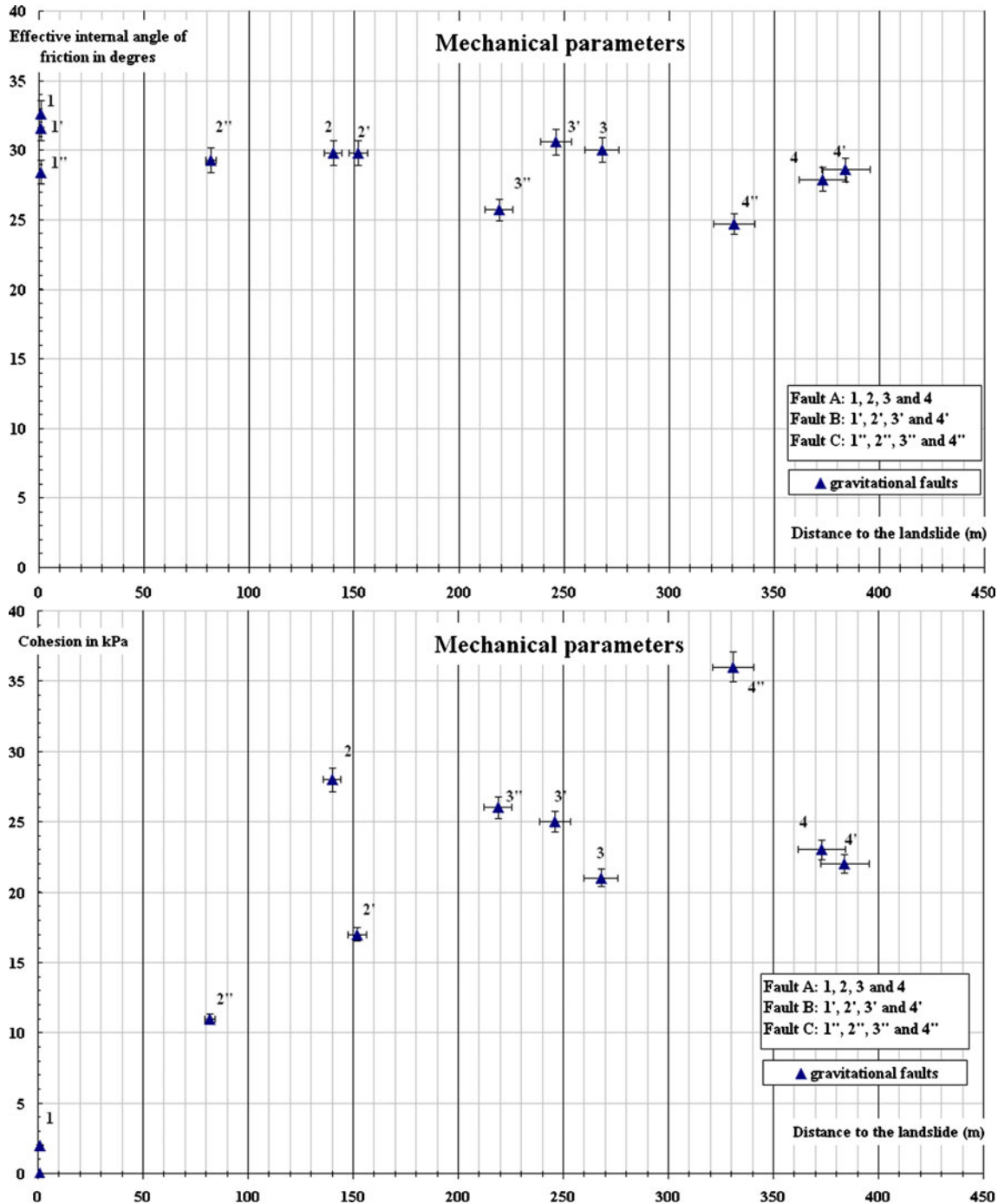
Fig. 7 Effective angle of internal friction ( \phi' ) in degree versus distance to the landslide and the effective cohesion ( c' ) in kilopascal versus distance to the landslide
