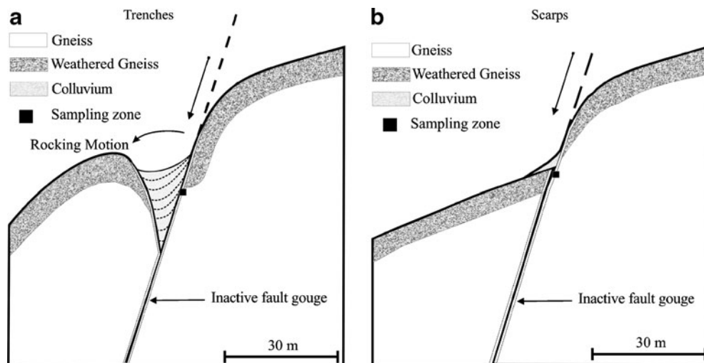
Fig. 2 a Schematic representation of the trenches. b Schematic representation of the scarps, with the structuration of the gneiss, weathered gneiss and colluviums material
